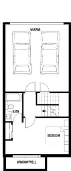
BASEMENT FLOOR - 384 SF GARAGE - 413 SF
