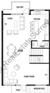
FIRST FLOOR 969 SF
