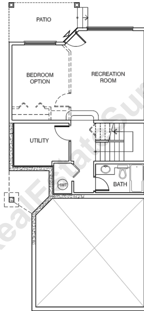
GROUND LEVEL
