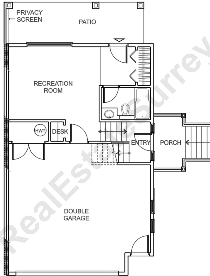
GROUND LEVEL
