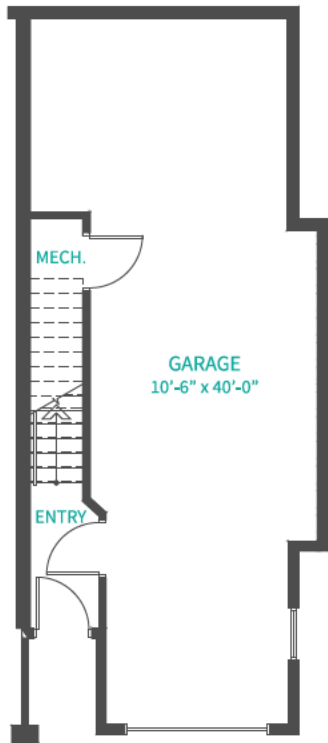
LOWER FLOOR 639 S.F.
