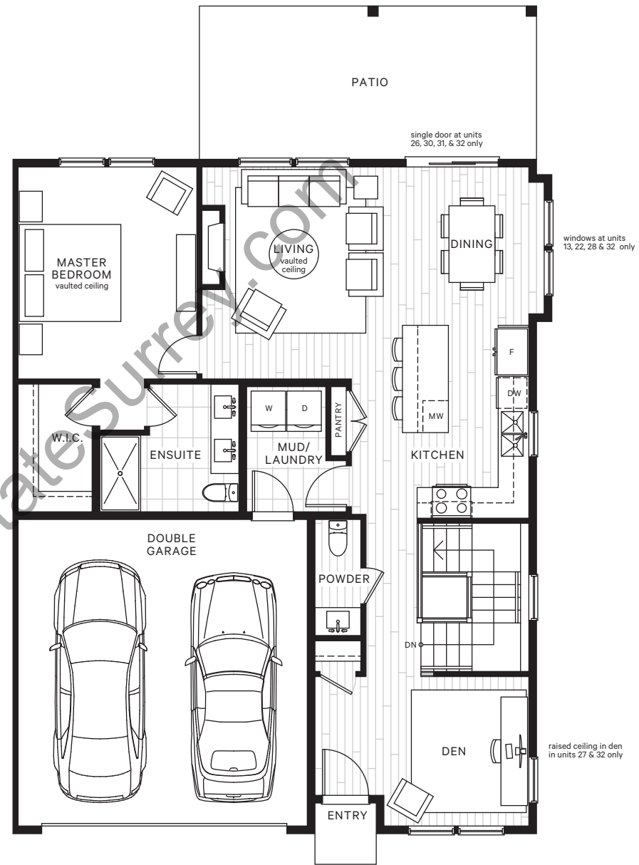
MAIN
