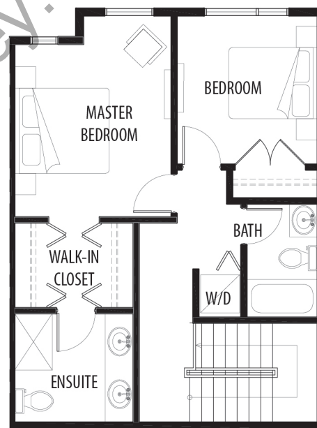
SECOND FLOOR 642 S.F.
