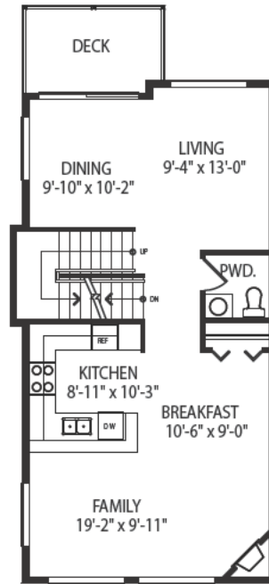
MAIN FLOOR PLAN 798 S.F. ( 74.14 m2 )
