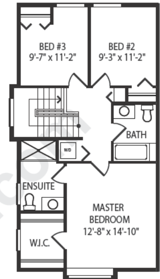
UPPER FLOOR PLAN 776 S.F. ( 72.09 m2 )
