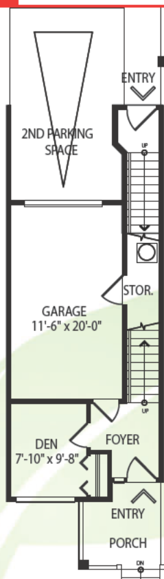
BASEMENT PLAN 250 S.F. ( 23.23 m2 )
