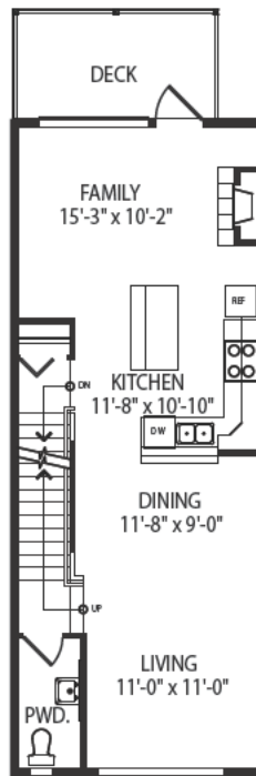
MAIN FLOOR PLAN 672 S.F. ( 62.43 m2 )
