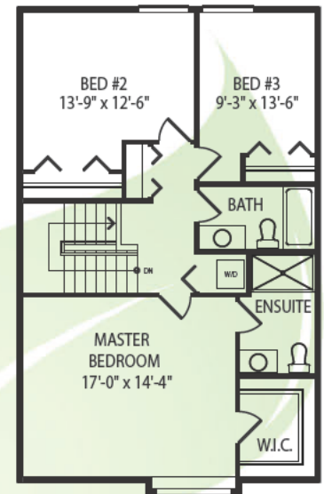
UPPER FLOOR PLAN 920 S.F. ( 85.47 m2 )
