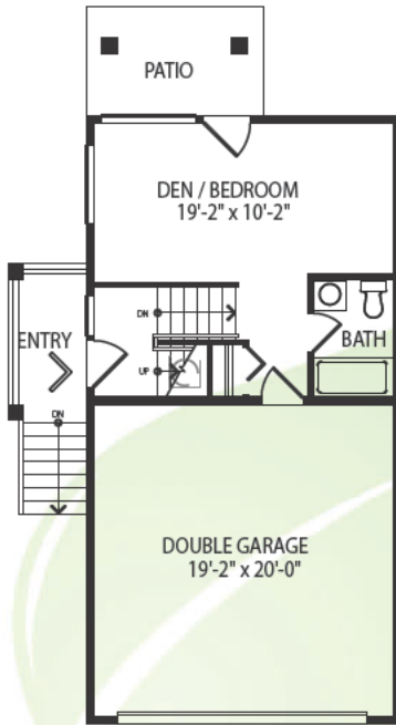
BASEMENT PLAN 370 S.F. ( 34.37 m2 )
