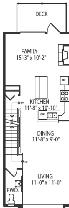
MAIN FLOOR PLAN 683 S.F. ( 63.45 m2 )
