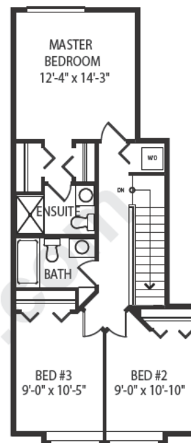
UPPER FLOOR PLAN 717 S.F. ( 66.61 m2 )
