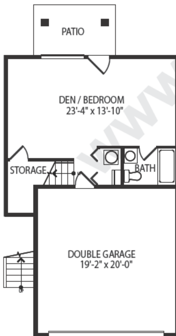
BASEMENT PLAN 461 S.F. ( 42.83 m2 )
